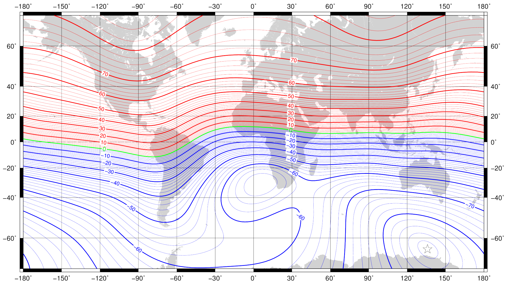
Inclination (magnetic dip) at 2020.0 from the World Magnetic Model (WMM2020). Red – positive (down), blue – negative (up), green – zero (dip equator). Contour interval is 2°, white star is location of a magnetic pole and projection is Mercator. This is an example of an isoclinic chart. Credit: British Geological Survey (UK Research and Innovation).
