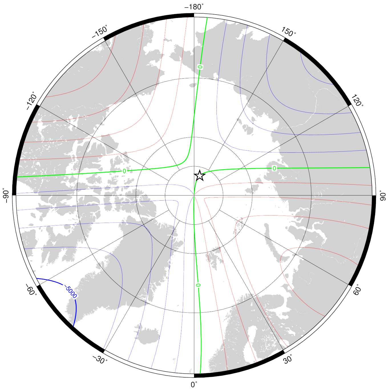
East component ( Y ) in region of north pole at 2020.0 from the World Magnetic Model (WMM2020). Red – positive (east), blue – negative (west), green – zero. Contour interval is 1000 nT, white star is location of a magnetic pole and projection is Polar Stereographic. Credit: British Geological Survey (UK Research and Innovation).
