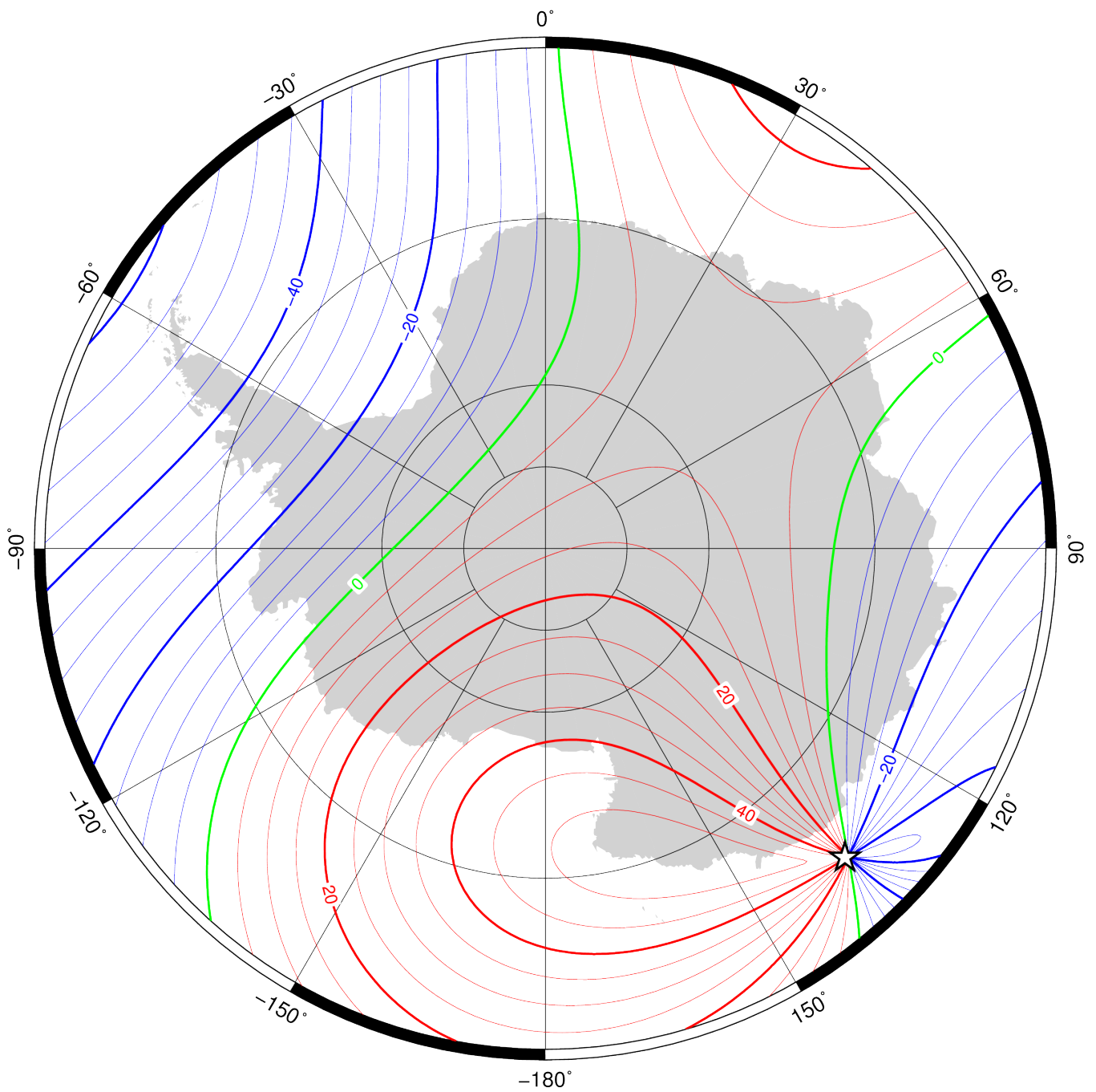
Annual rate of change of horizontal intensity in region of south pole for 2020.0 to 2025.0 from the World Magnetic Model (WMM2020). Red – positive change, blue – negative change, green – zero change. Contour interval is 5 nT/year, white star is location of a magnetic pole and projection is Polar Stereographic. Credit: British Geological Survey (UK Research and Innovation).
