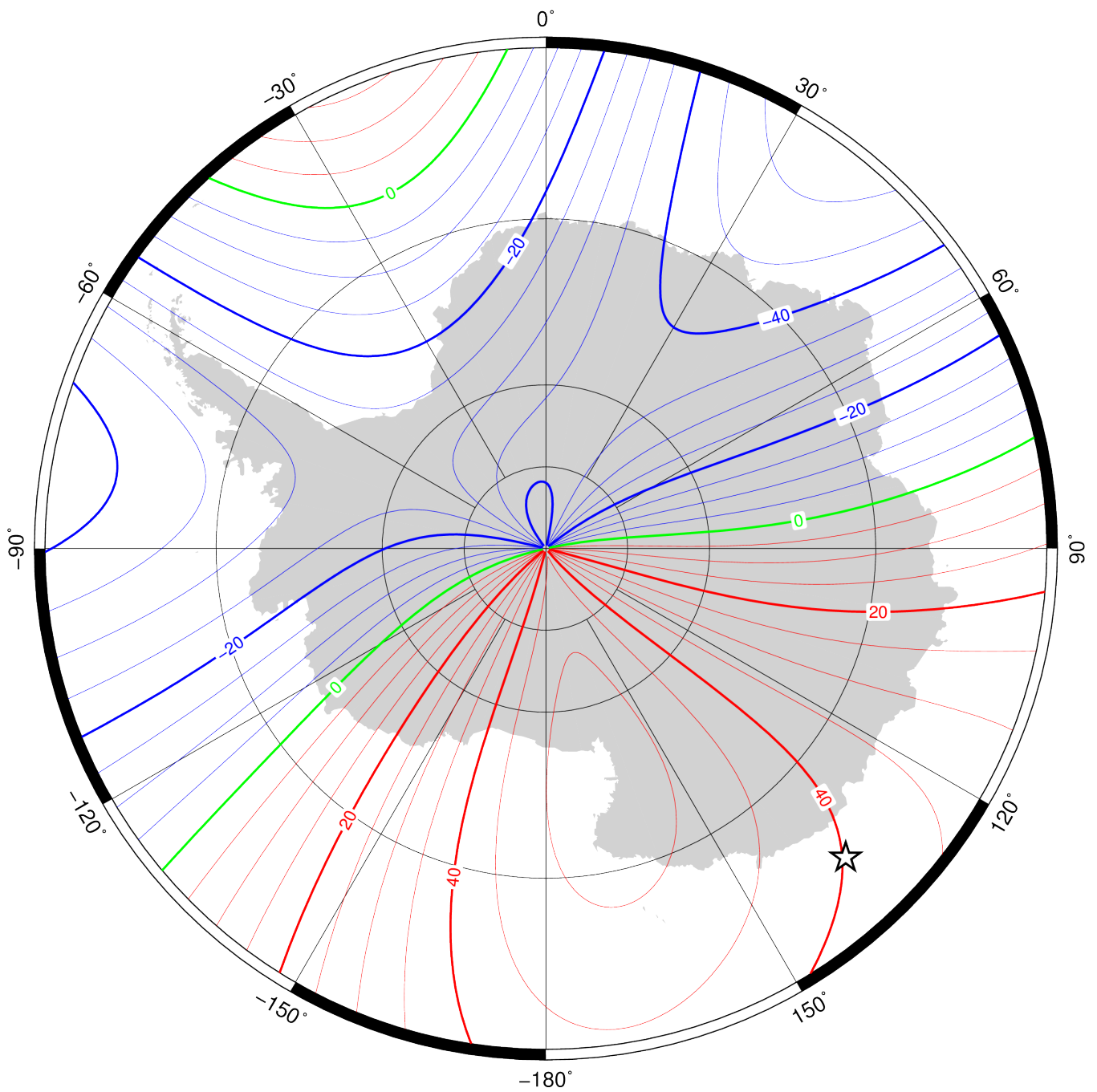
Annual rate of change of east component in region of south pole for 2020.0 to 2025.0 from the World Magnetic Model (WMM2020). Red – positive change, blue – negative change, green – zero change. Contour interval is 5 nT/year, white star is location of a magnetic pole and projection is Polar Stereographic. Credit: British Geological Survey (UK Research and Innovation).
