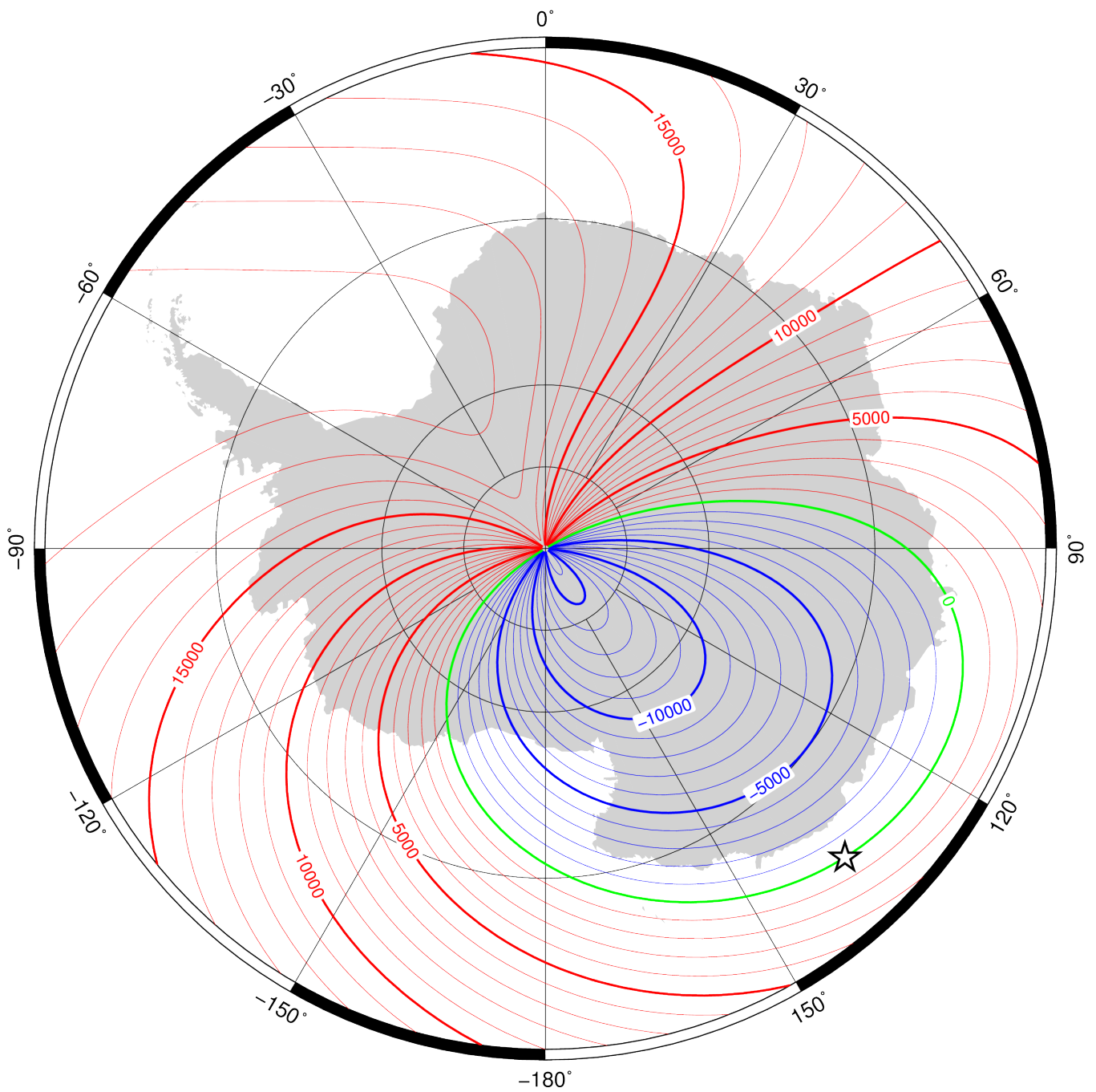
North component ( X ) in region of south pole at 2020.0 from the World Magnetic Model (WMM2020). Red – positive (north), blue – negative (south), green – zero. Contour interval is 1000 nT, white star is location of a magnetic pole and projection is Polar Stereographic. Credit: British Geological Survey (UK Research and Innovation).
